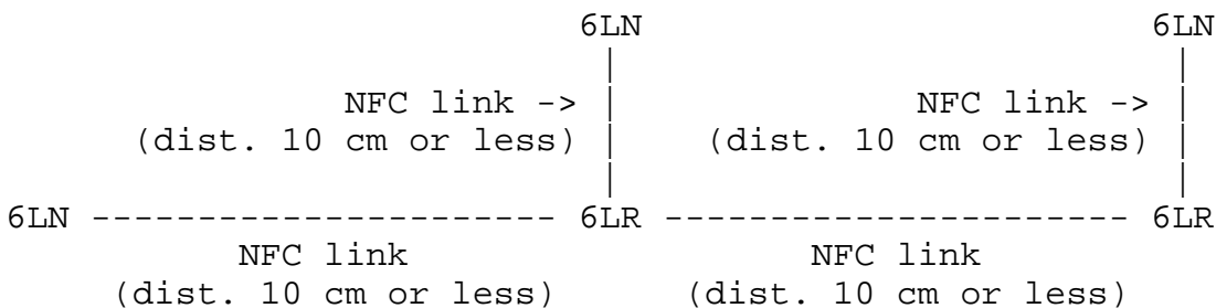
Figure 11: Isolated NFC-enabled device network
