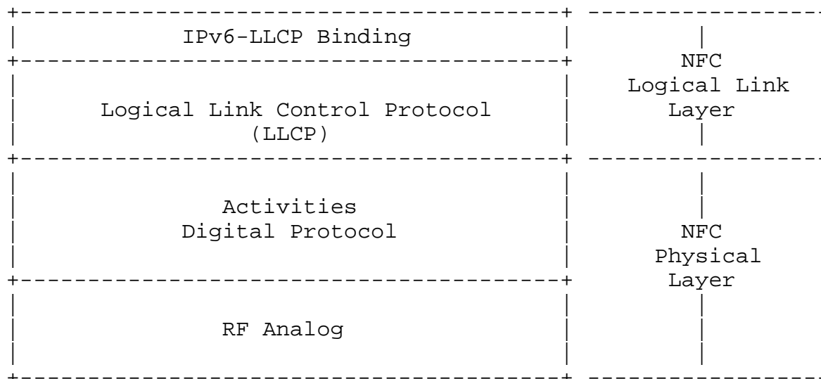
Figure 1: Protocol Stack of NFC
