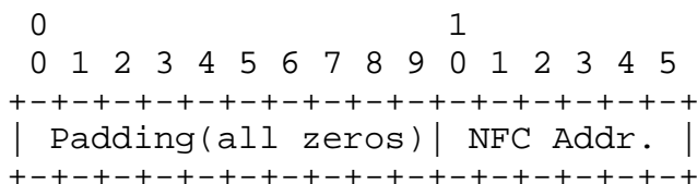
Figure 8: NFC short address format
