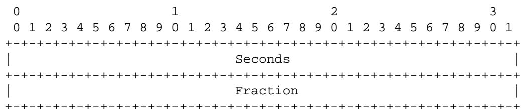
Figure 2: NTP [RFC5905] 64-bit Timestamp Format
