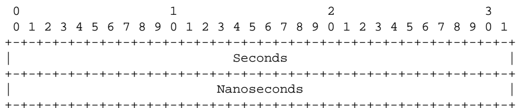
Figure 1: PTP [ IEEE1588v2 ] Truncated Timestamp Format
