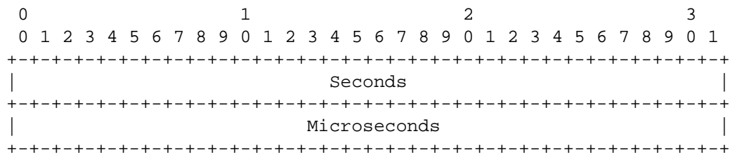
Figure 3: POSIX-based Timestamp Format
