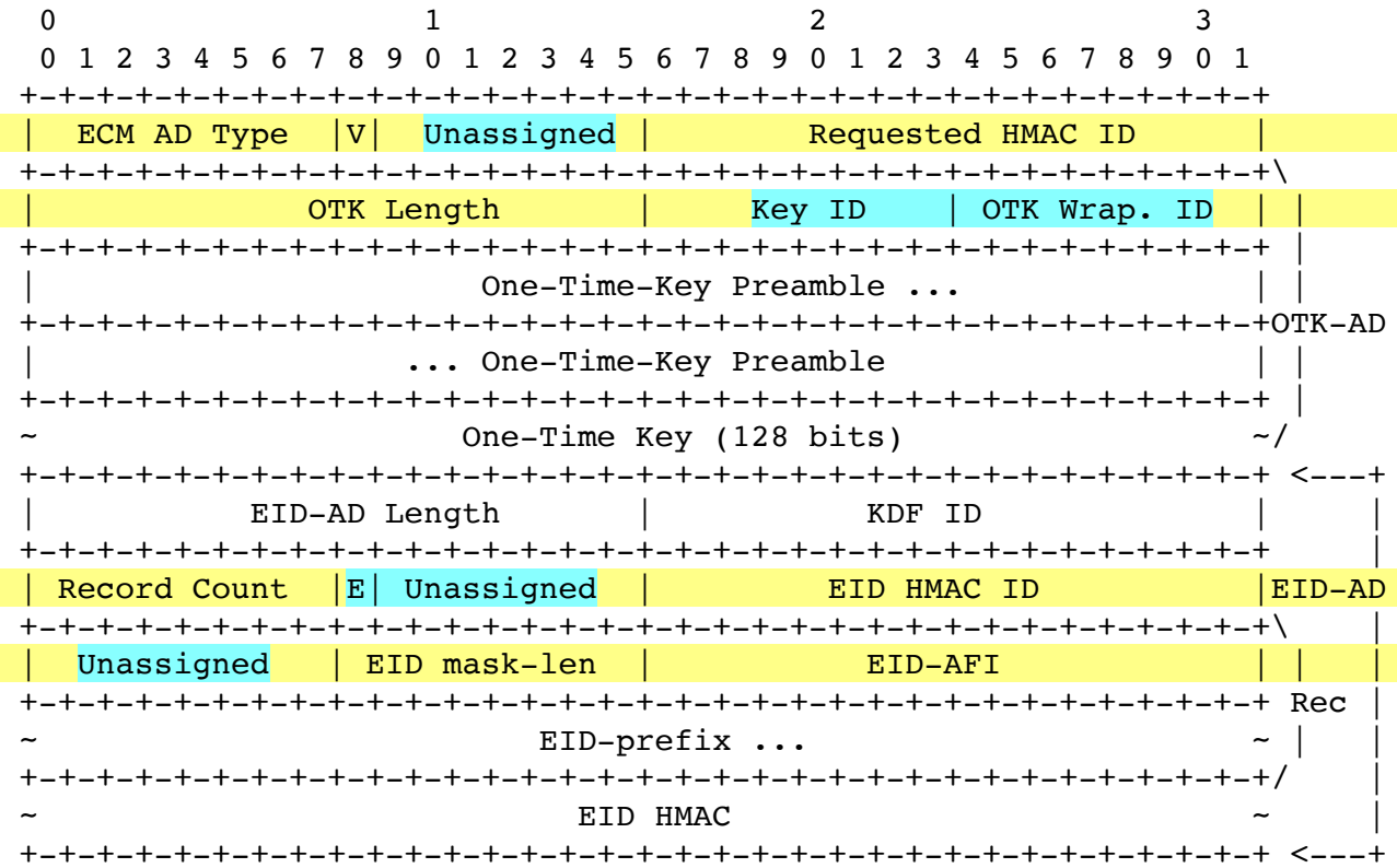
Figure 1: LISP-SEC ECM Authentication Data
