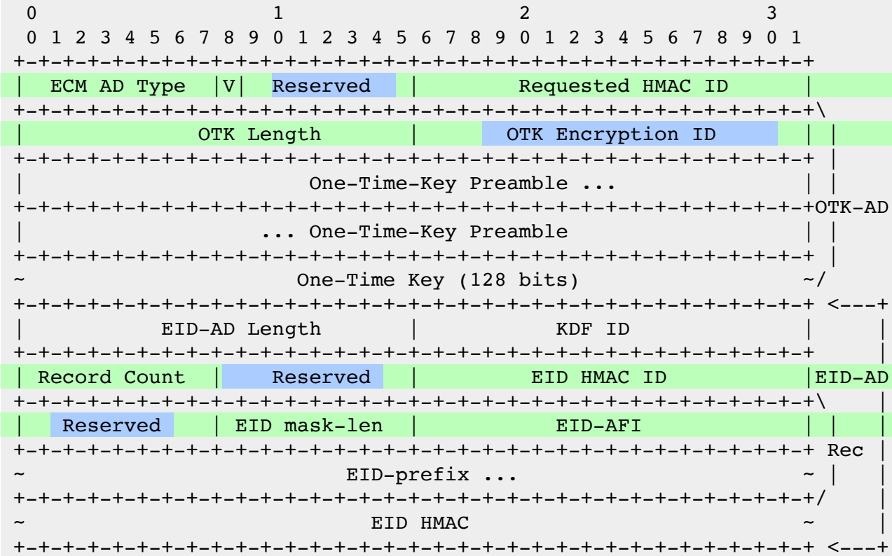
LISP-SEC ECM Authentication Data
