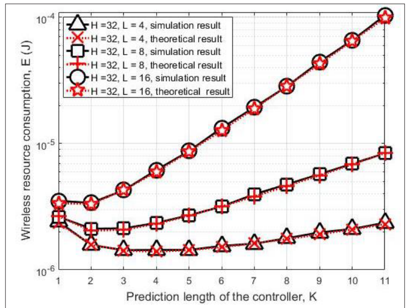
Figure 4. The relationship between the resource consumption E in the wireless communication network and the prediction length K in the control system, where H and L represent the numbers of bits for the header and payload of a communication packet, respectively.
