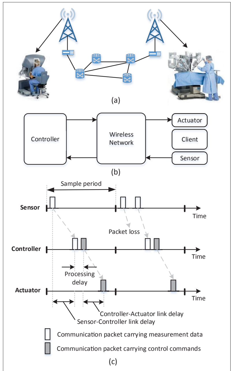
Figure 1. A typical real-time wireless control system: a) the use case of remote surgery; b) system diagram; c) timing diagram of the wireless communication.
