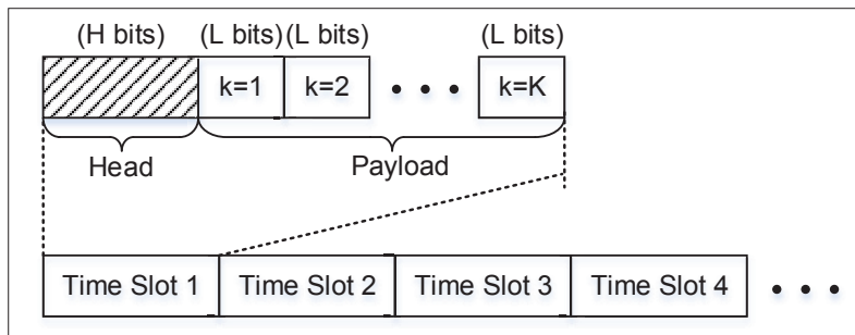
Figure 3. Communication frame structure for the controller-actuator link in PPC.
