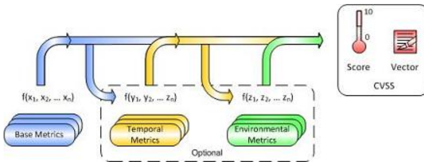
Figure 2: CVSS Metrics and Equations
