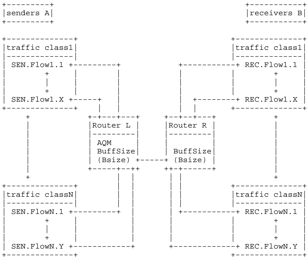
Figure 1: Topology and notations
